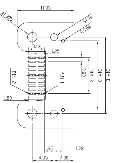
RECOMMENDED PCB LAYOUT TOLERANCE:±0.05
